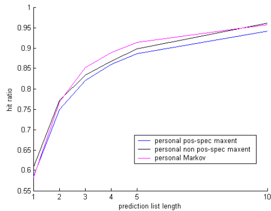
Figure 4: Hit Ratio Results of Personalized Mixture Models on All Users for 10 Components.
