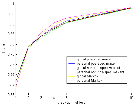
Figure 1: Hit Ratio Results on Known Users For 3 Component Mixture Model.
