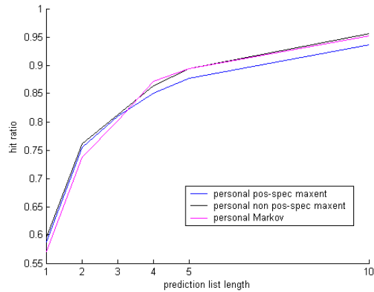
Figure 3: Hit Ratio Results of Personalized Mixture Models on All Users for 3 Components.
