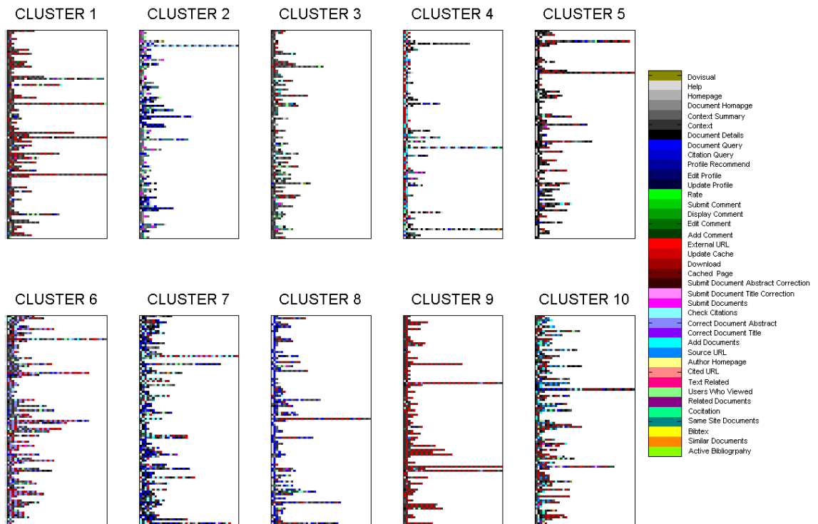
Figure 6: User Clusters Generated by the 10-Component Markov Mixture Model.
