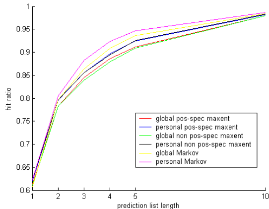
Figure 2: Hit Ratio Results on Known Users For 10 Component Mixture Model.
