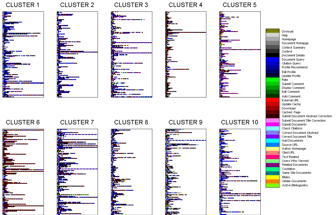
Figure 7: User Clusters Generated by the 10-Component Non Position Specific Maximum Entropy Mixture Model.
